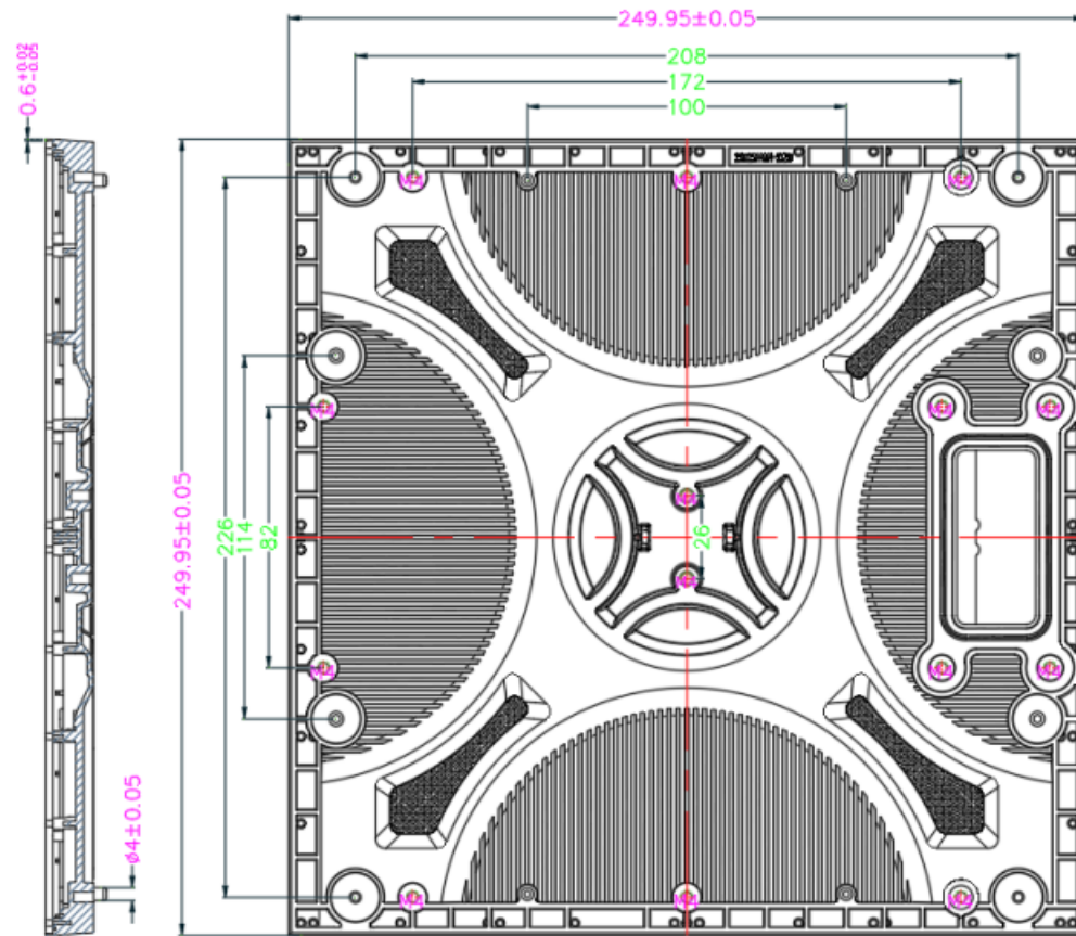
Picture 4-1 Hole Installation Diagram for Kit
