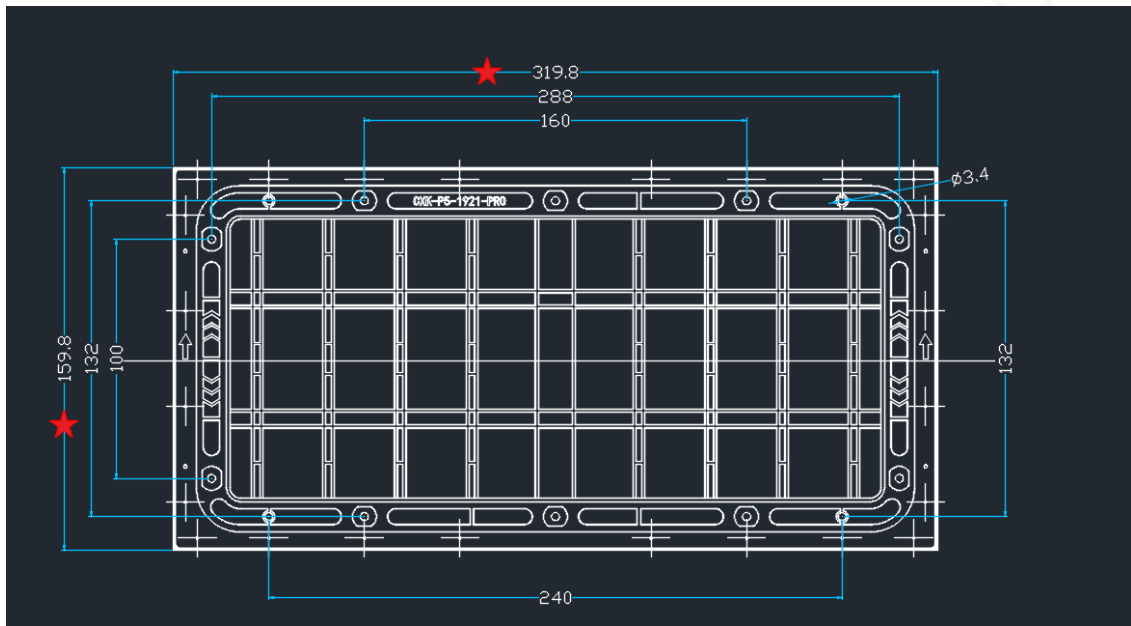
Picture 4-1 Hole Installation Diagram for Kit
