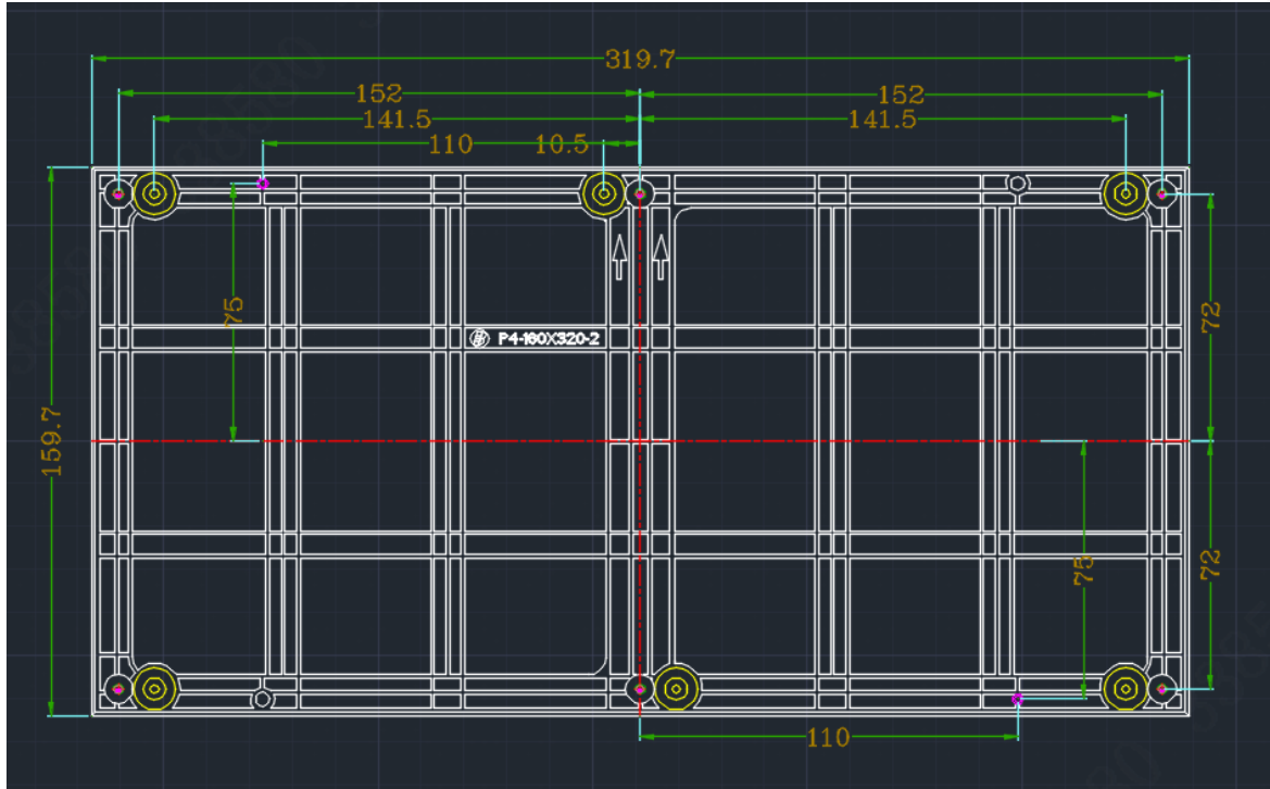
Picture 4-1 Hole Installation Diagram for Kit
